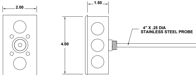
Duct/Immersion sensor shown without box.
